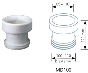
Straight drainage pipe for diameter matching adjustment (92 000607)
